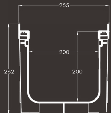
TYPE 200/200
